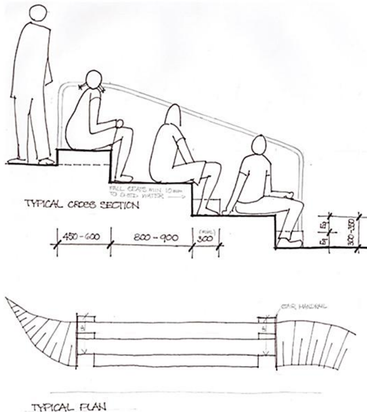
Figure 01: Typical Cross Section and Typical Plan
