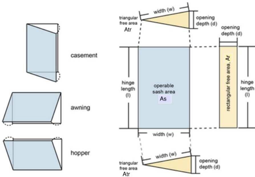
Figure 7.7.1 Awning Window Area
