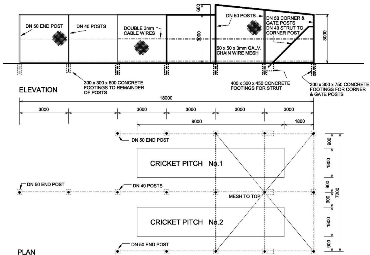
Figure 02: Batting Practice Nets
