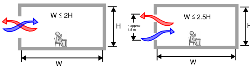
Figure 7.7.2 Single Sided Opening(s)
