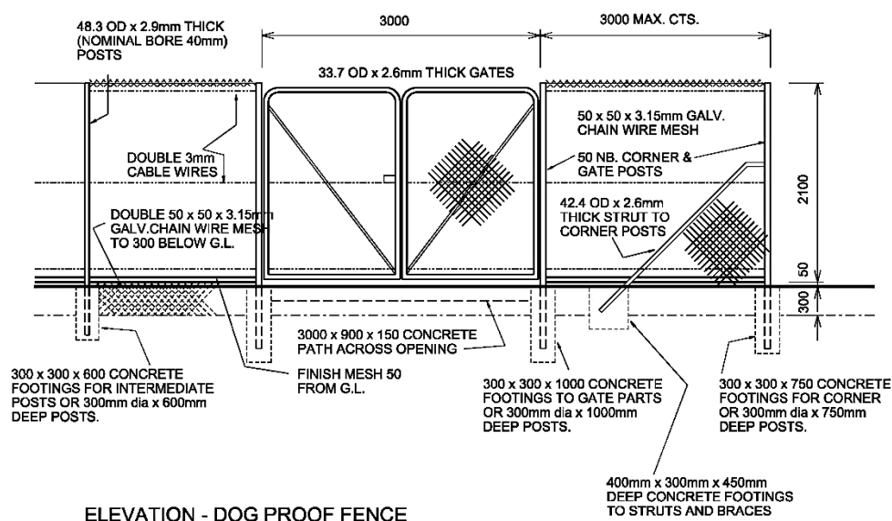
Figure 02: Dog Proof Enclosing Fence – Secondary
