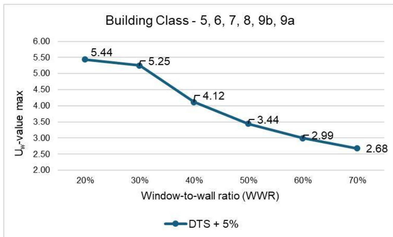
Figure 2.1.1 Building glazing U_w values against window to wall ratio (WWR)
