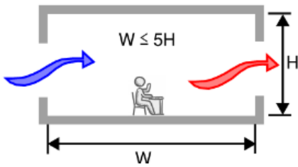
Figure 7.7.3 Cross Ventilation Openings
