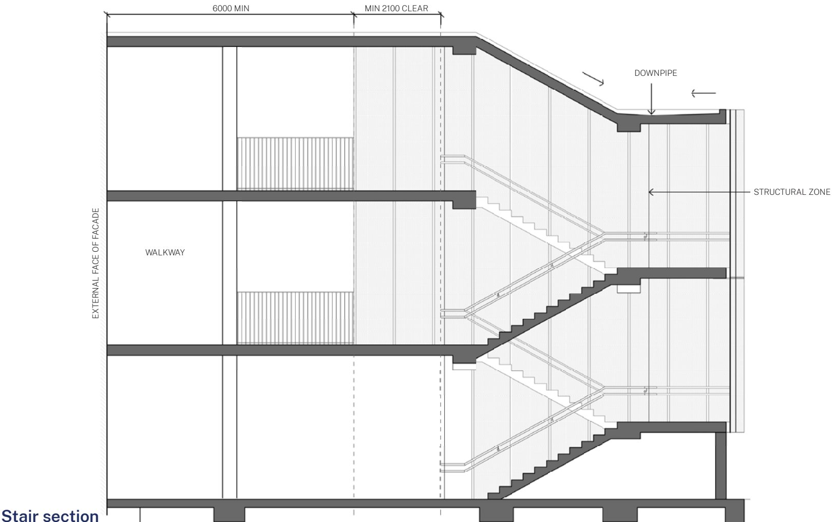
Stair section
