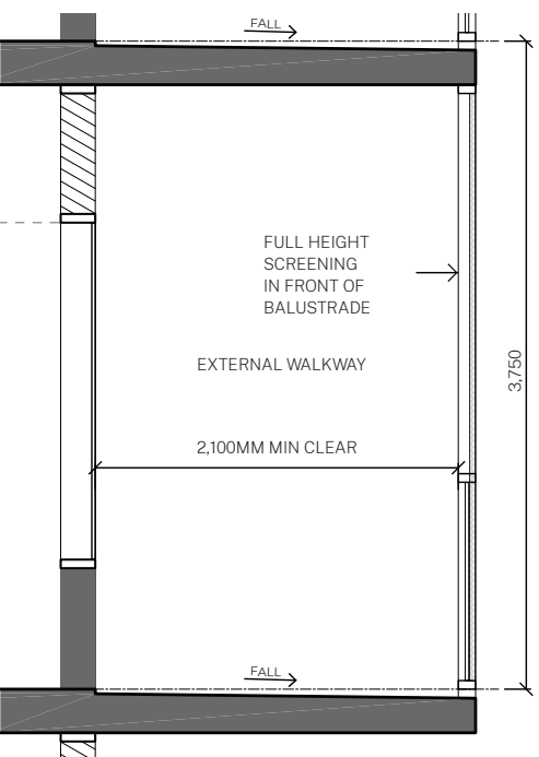
Section
