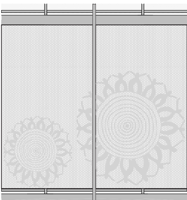
Elevation - perforated screening
