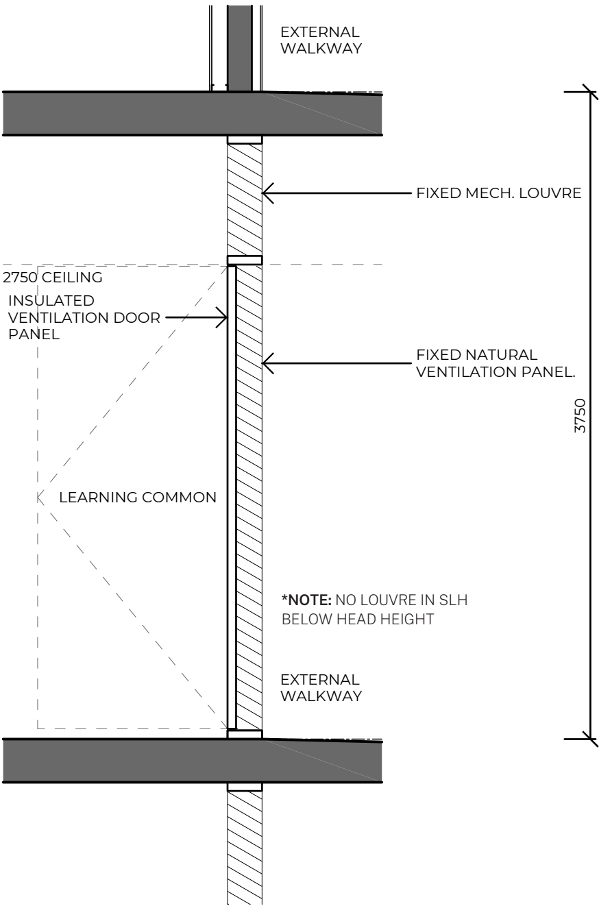
Walkway side ventilation panel section
