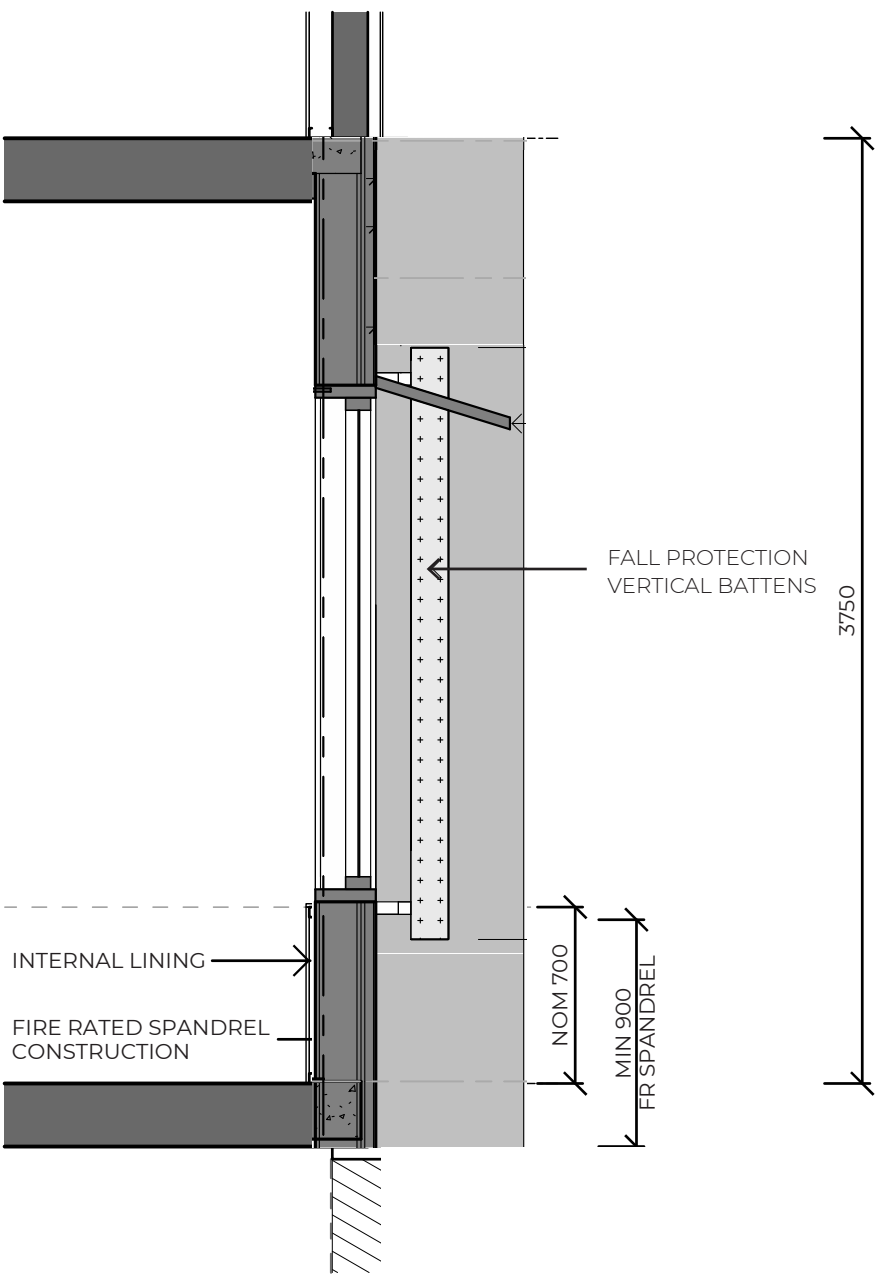
Street side ventilation panel with fixed louvre section
