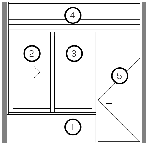
Panel Type 2
