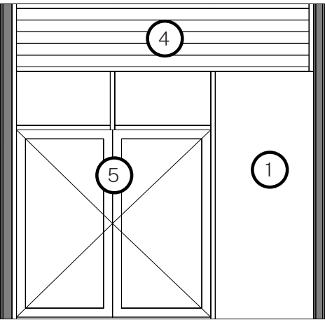
Panel Type 1
