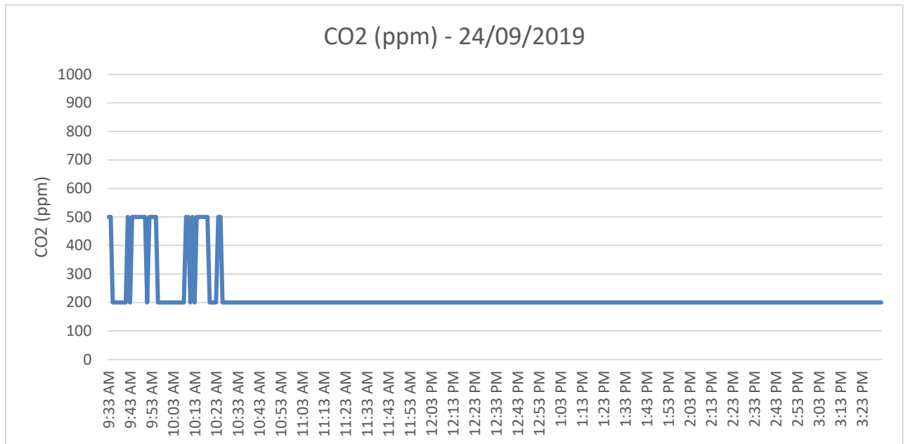
Figure 1: Carbon Dioxide (CO 2 ) monitoring results
