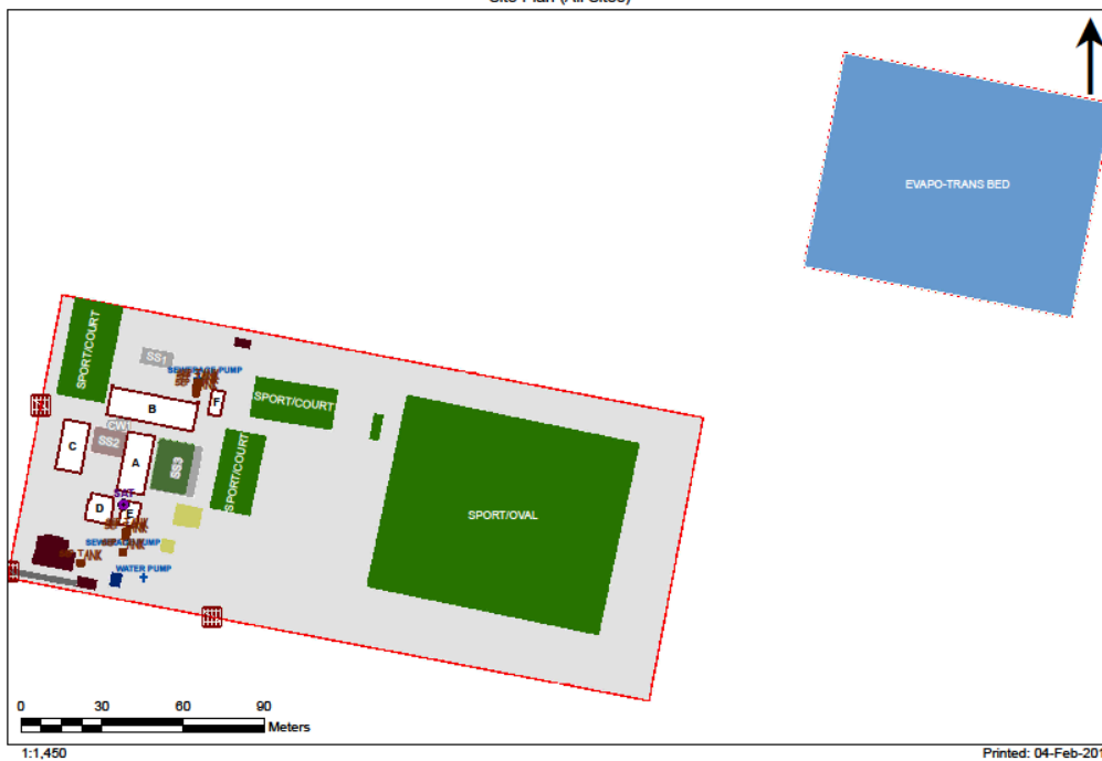
2827 - Pallamallawa Public School Site Plan (All Sites)
