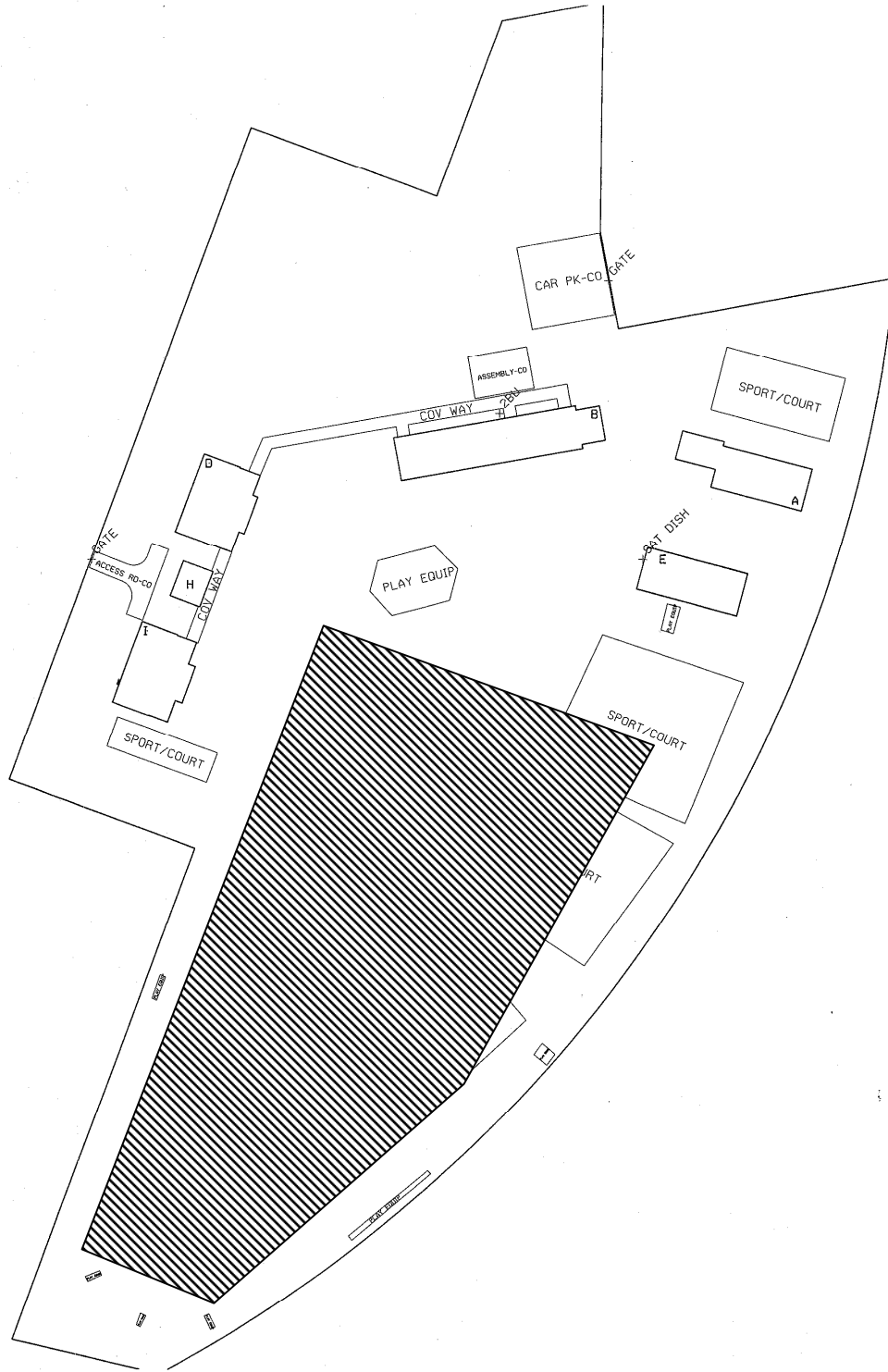
Figure 1. Woonona East Public School – site plan
